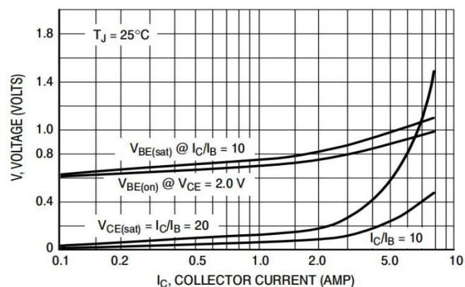
Figure 4. "On" Voltage
