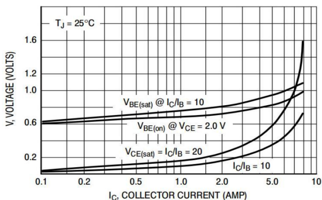
Figure 4. "On" Voltage
