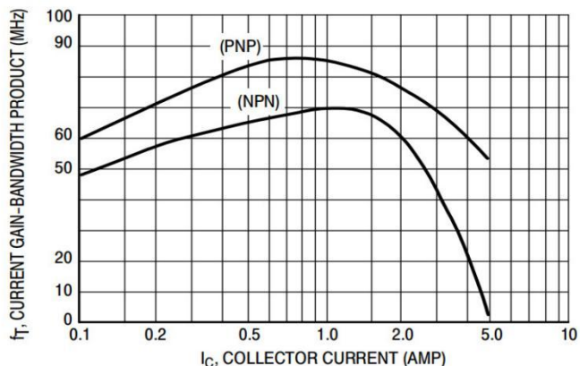
Figure 2. Current Gain-Bandwidth Product
