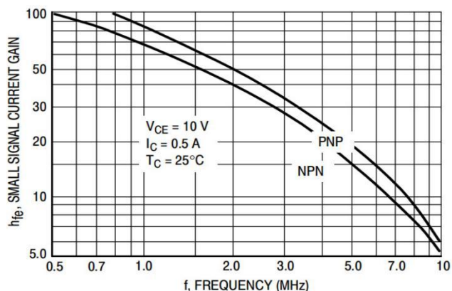
Figure 1. Small-Signal Current Gain
