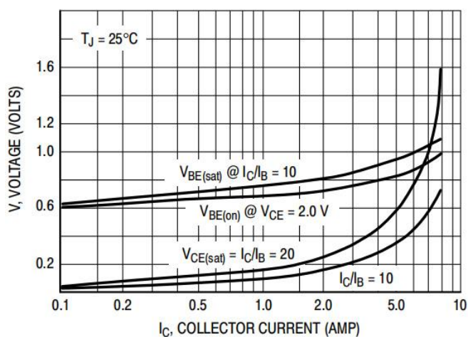
Figure 6. "On" Voltage
