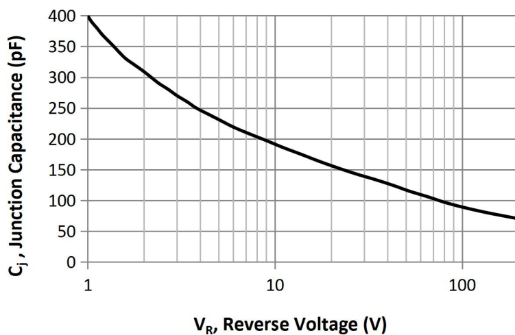
FIG.7 Junction Capacitance vs. Reverse Voltage
