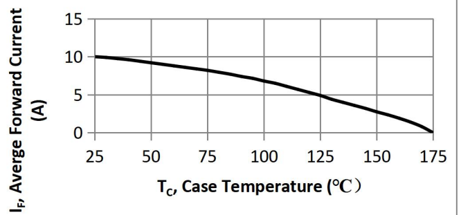
FIG.6 Average Forward Current vs. Case Temperature
