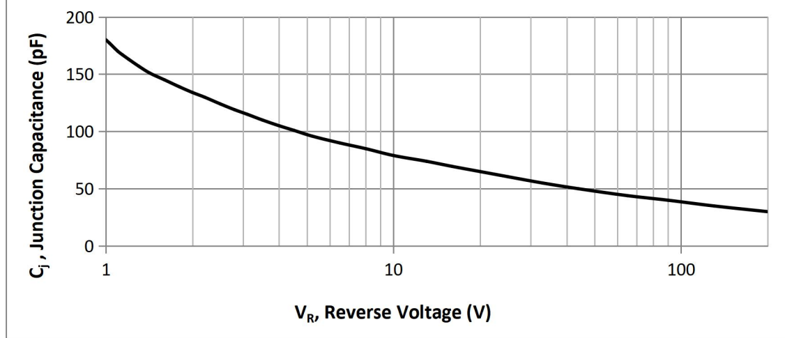
FIG.7 Junction Capacitance vs. Reverse Voltage
