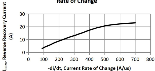
FIG.5 Reverse Recover Current vs. Current Rate of Change
