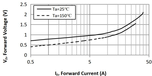
FIG.1 Forward Characteristic (typical)
