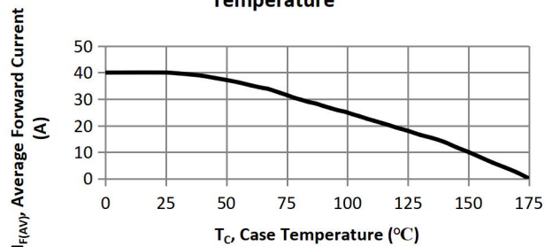
FIG.6 Average Forward Current vs. Case Temperature
