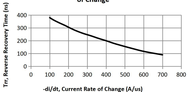
FIG.3 Reverse Recover Time vs. Current Rate of Change
