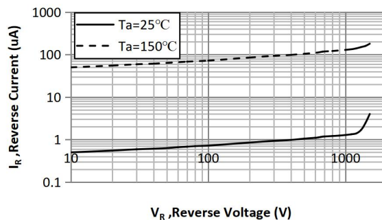
FIG.2 Reverse Characteristic (typ.)
