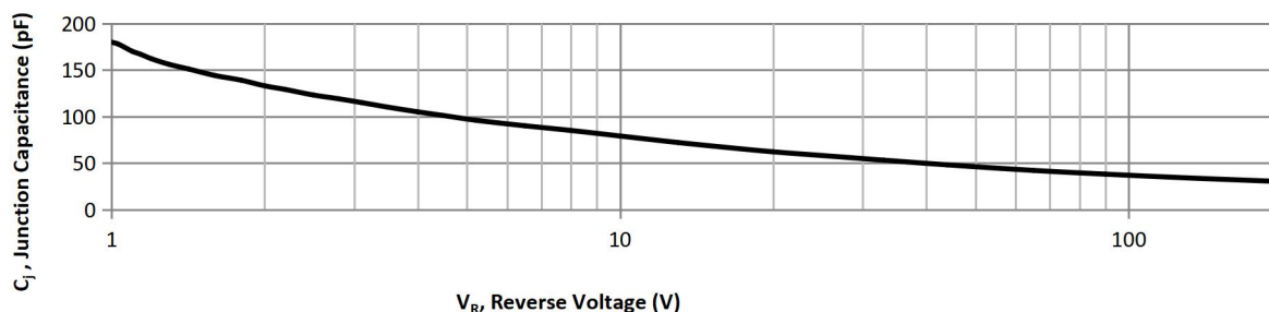
FIG.7 Junction Capacitance vs. Reverse Voltage
