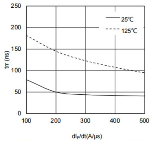
Figure 2. Reverse Recovery Time vs dI_F/dt
