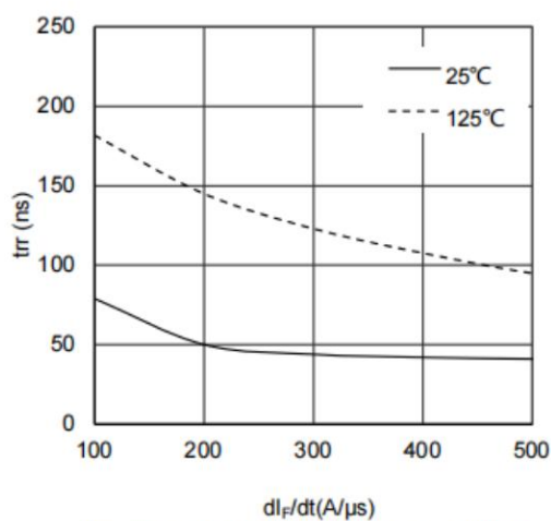
Figure 2. Reverse Recovery Time vs dI_F/dt
