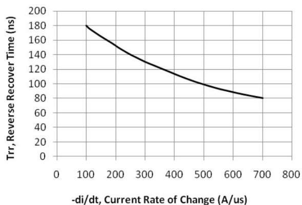
FIG.3 Reverse Recover Time vs. Current Rate of Change
