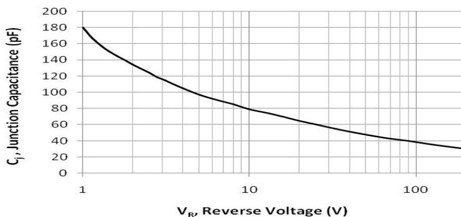
FIG.7 Junction Capacitance vs. Reverse Voltage
