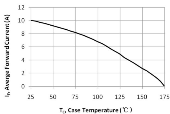
FIG.6 Average Forward Current vs. Case Temperature
