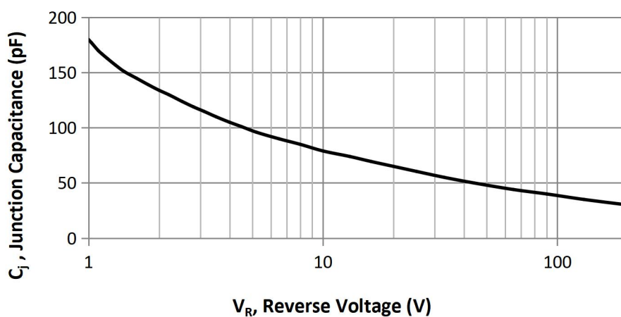
FIG.7 Junction Capacitance vs. Reverse Voltage
