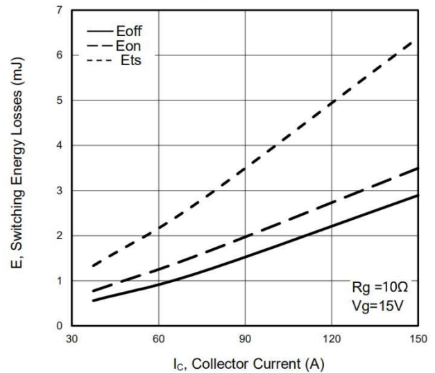
Figure 14 Switching Loss vs. Collector Current
