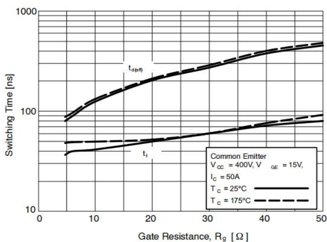
Figure 10. Turn-Off Characteristics vs. Gate Resistance
