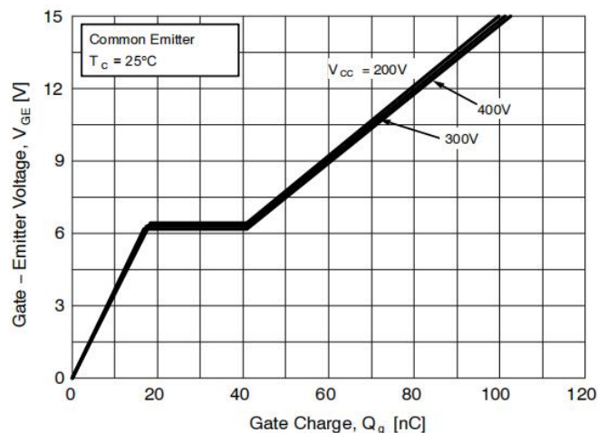
Figure 8. Gate Charge
