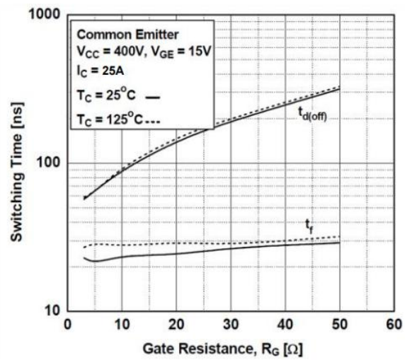
Figure 8. Turn-Off Characteristics vs. Gate Resistance
