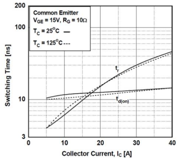
Figure 10. Turn-On Characteristics vs. Collector Current
