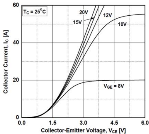
Fig 1. Output characteristics
