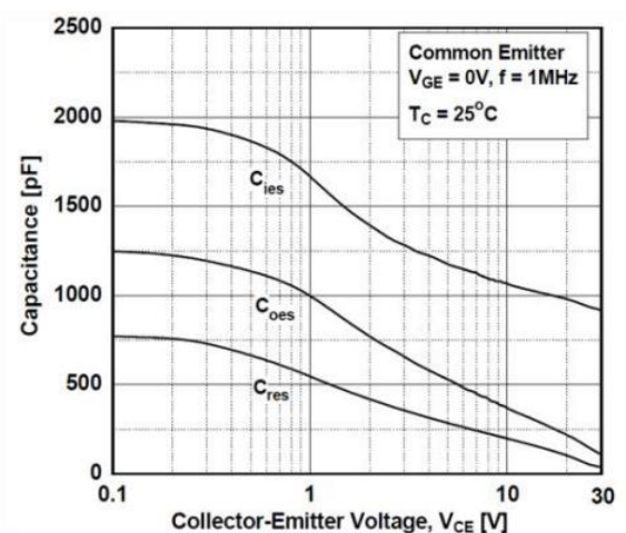
Figure 6. Capacitance Characteristics
