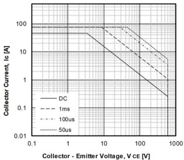
Figure 14. SOA Characteristics
