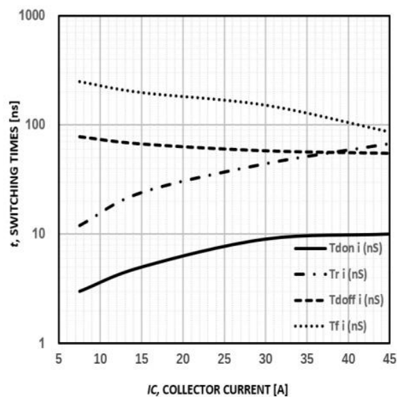
Figure 8 : typical switching time VS. IC, TC=25°C,
