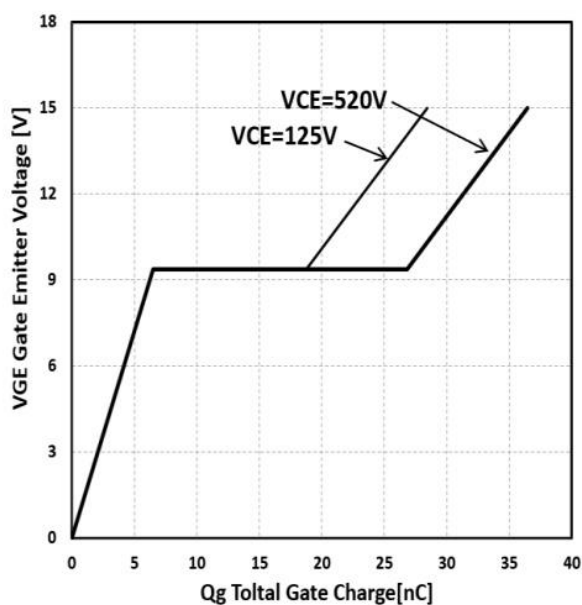
Figure 6 :typical gate charge VS. VGE,IC=15A
