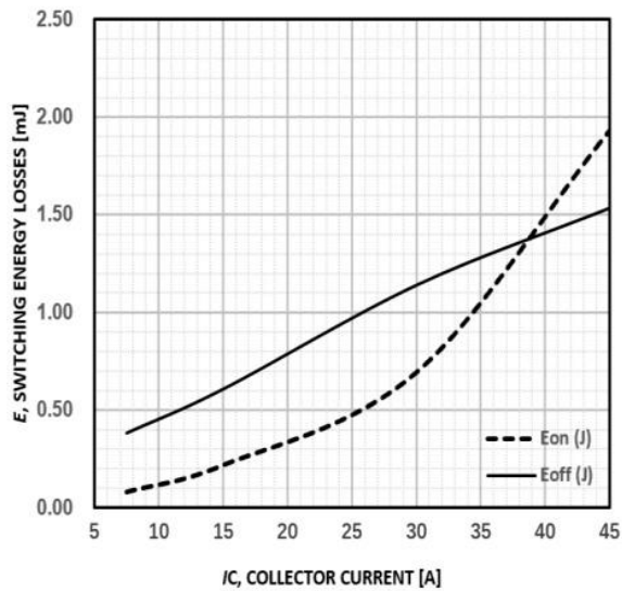
Figure 9 : typical energy loss VS. IC, TC=125°C,
