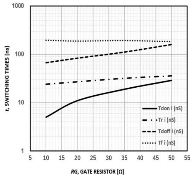
Figure12: typical switching time VS. Rg,TC=25°C,
