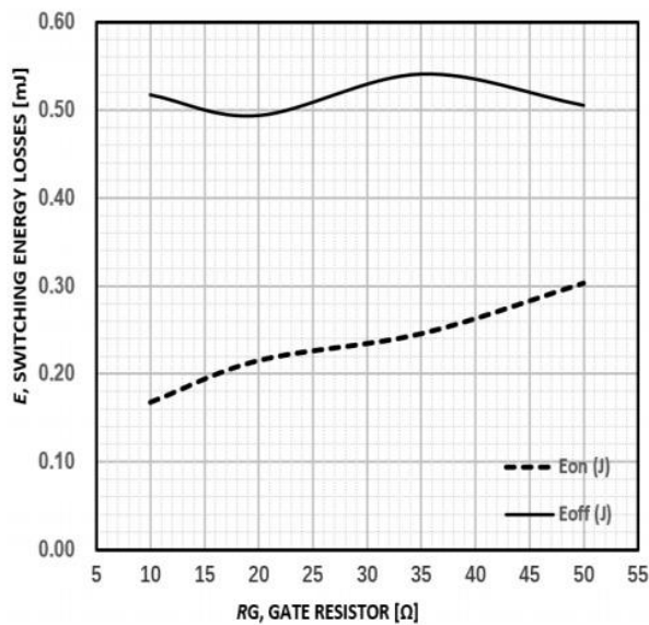
Figure11: typical energy loss VS. Rg,TC=25°C,
