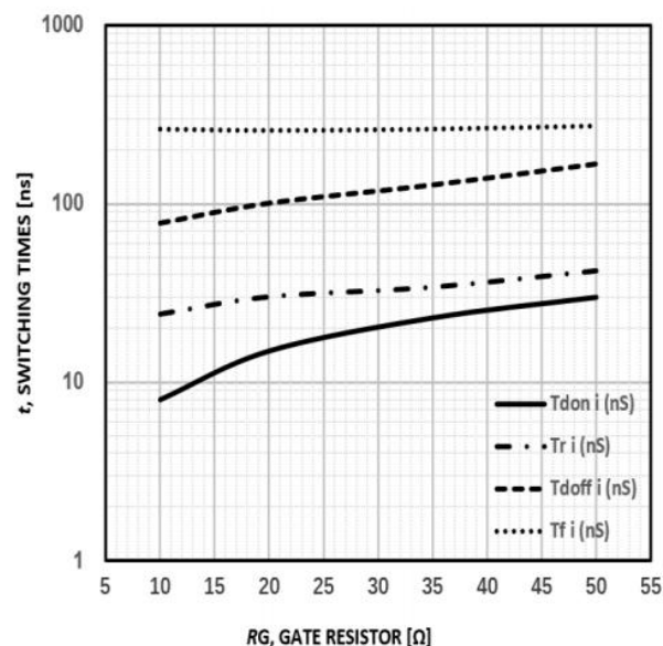
Figure14: typical switching time VS. R_g , T_C=125^{\circ}\text{C} , L=500\mu\text{H} , V_{CE}=400\text{V} , V_{GE}=15\text{V} , I_C=15\text{A}
