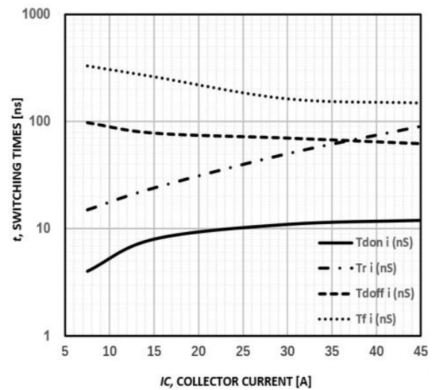
Figure10: typical switching time VS. IC, TC=125°C,
