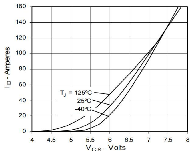
Fig 3: Input Admittance
