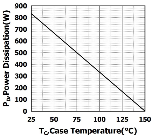
Fig 5: Power Dissipation
