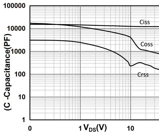
Fig 4: Capacitance Characteristics
