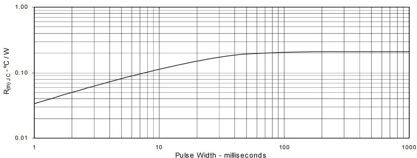
Fig 7: Maximum Transient Thermal Resistance
