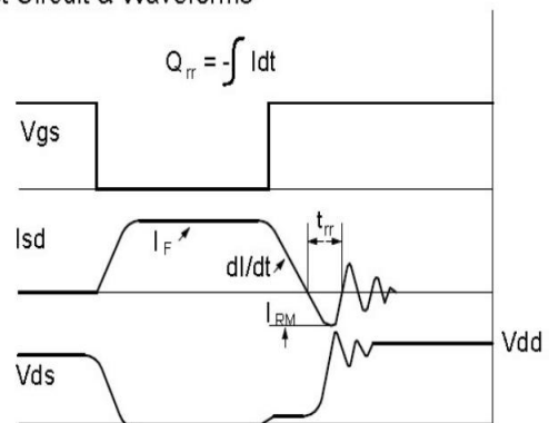
Diode Recovery Test Circuit & Waveforms
