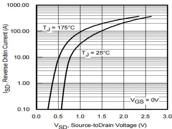
Fig 9: Typical Source-Drain Diode Forward Voltage
