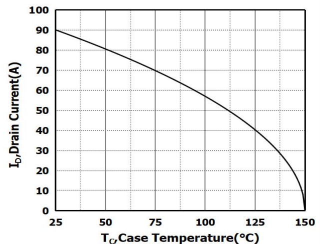
Fig 8: Drain Current Derating
