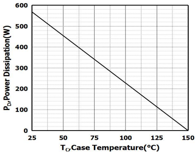
Fig 7: Power Dissipation
