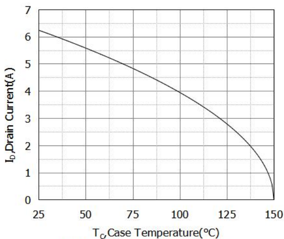
Figure 3. Id vs Case Temperature
