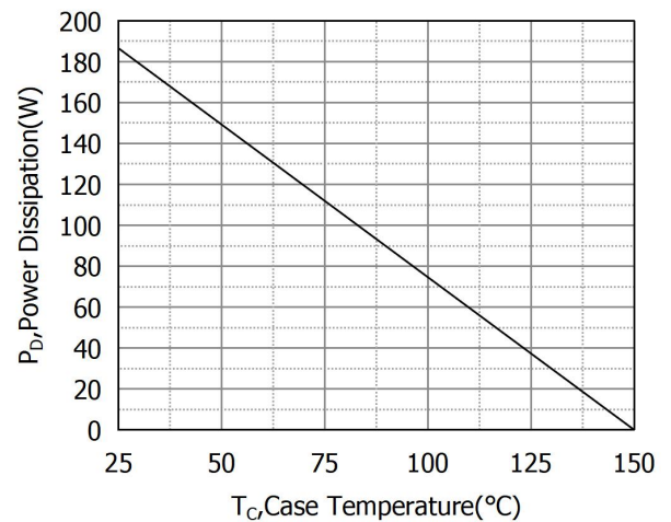
Figure 2. Maximum Power Dissipation vs Tc
