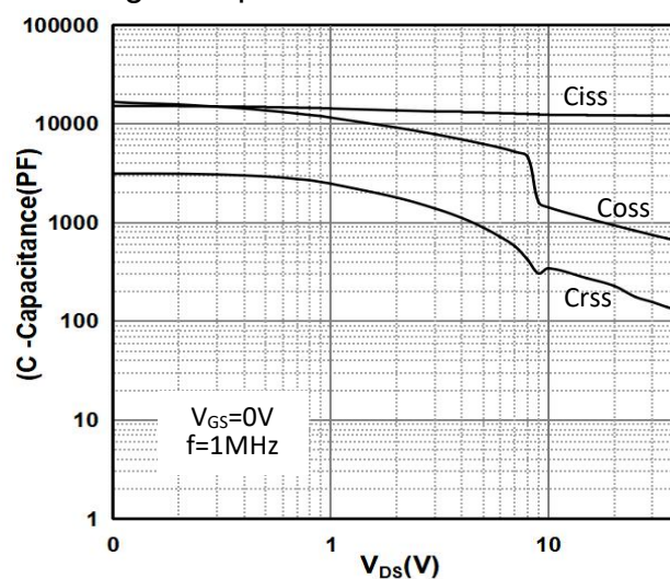
Fig 4: Capacitance Characteristics
