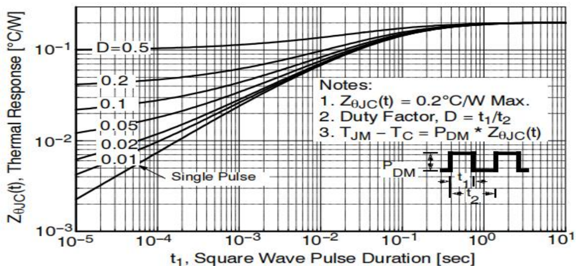
Fig 8: Max. Transient Thermal Impedance
