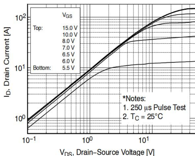
Fig 1: Output Characteristics
