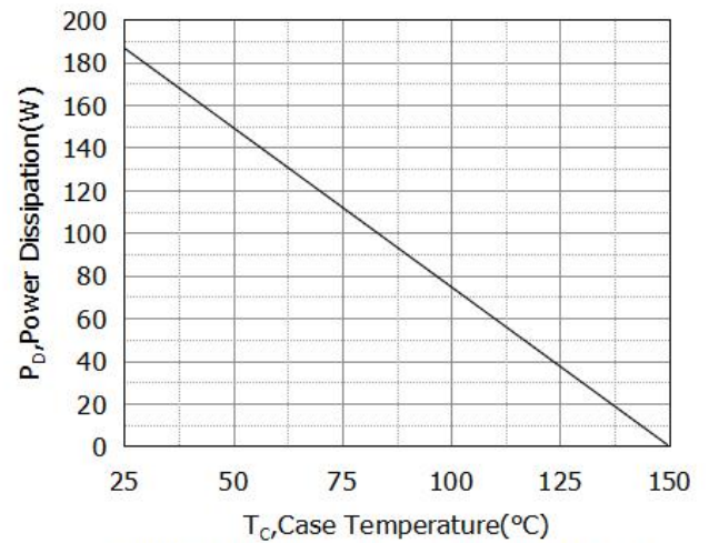
Figure 2. Maximum Power Dissipation vs Tc
