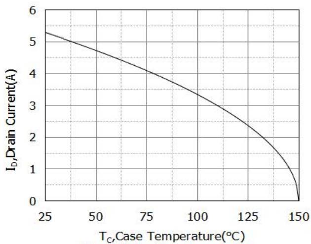
Figure 3. Id vs Case Temperature
