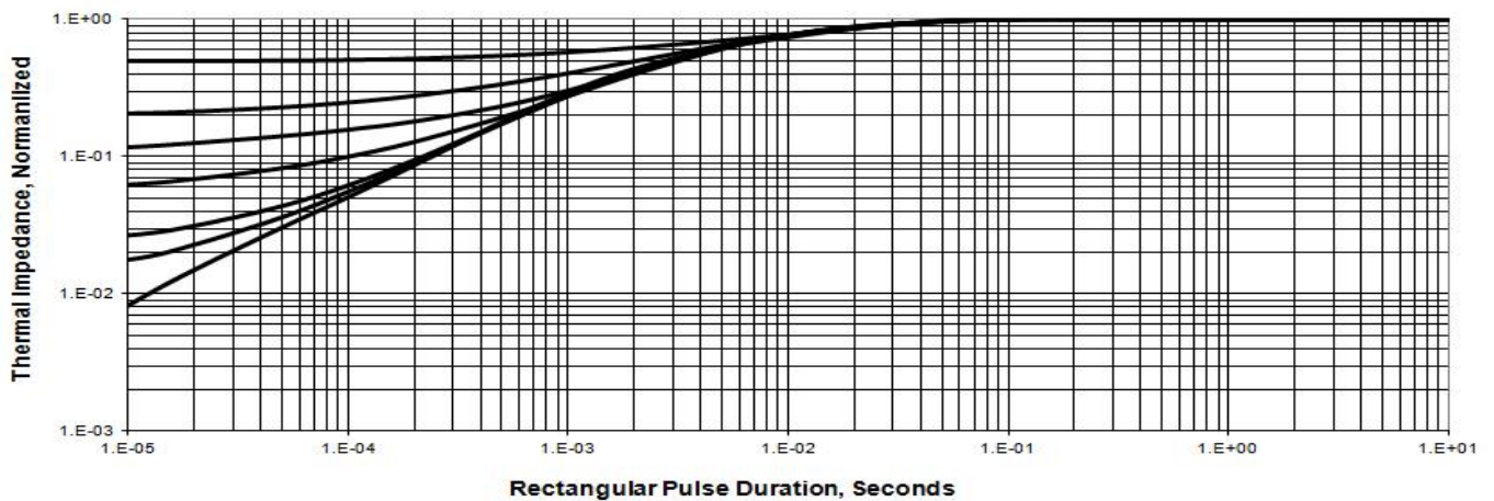
Figure 5. Maximum Transient Thermal Impedance
