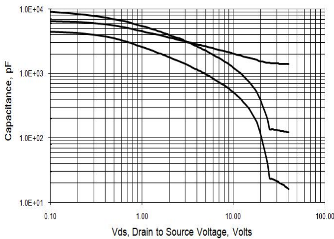
Figure 13. Capacitance vs Vds
