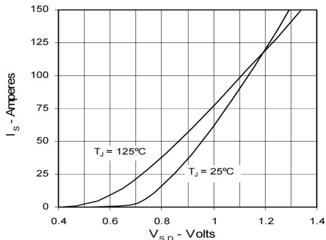
Fig 4: Source Current vs. Source-To-Drain Voltage
