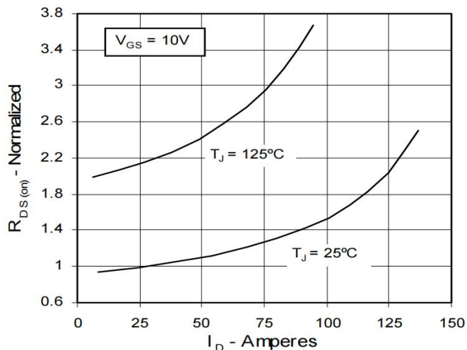
Fig 3: R_{DS(on)} Normalized to I_{D25} Value vs. I_D
