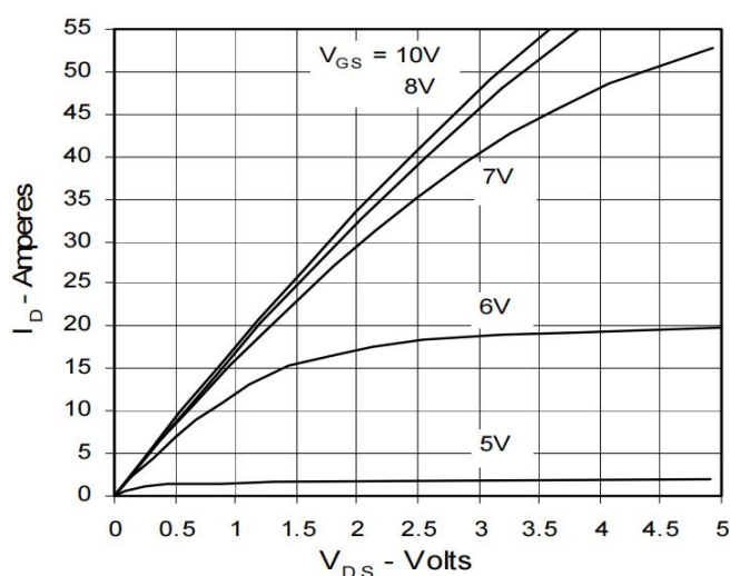
Fig 1: Output Characteristics
