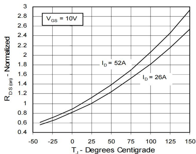
Fig 2: R_{DS(on)} Normalized to I_{D25} Value vs. Junction Temperature
