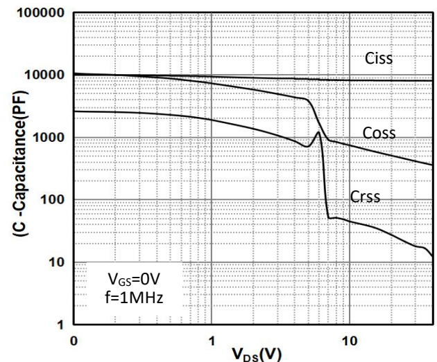
Fig 4: Capacitance Characteristics
