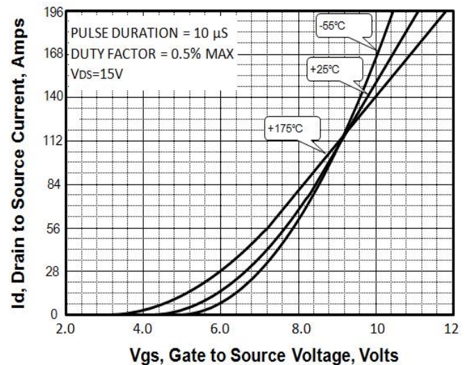
Fig 2: Transfer Characteristics
