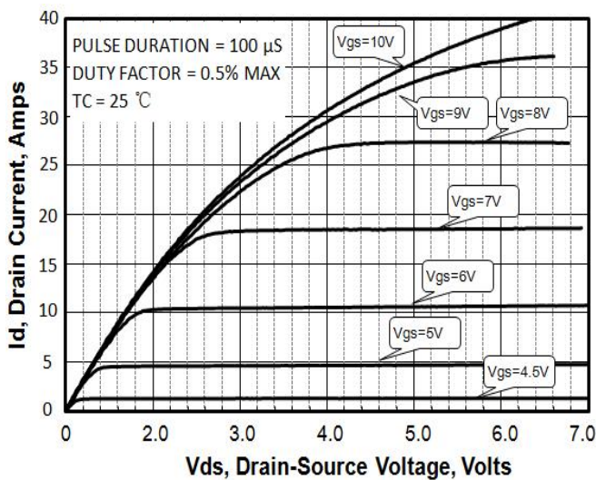
Fig 1: Output Characteristics
