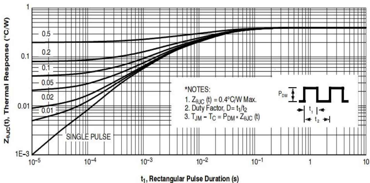
Fig 12: Transient Thermal Response Curve
