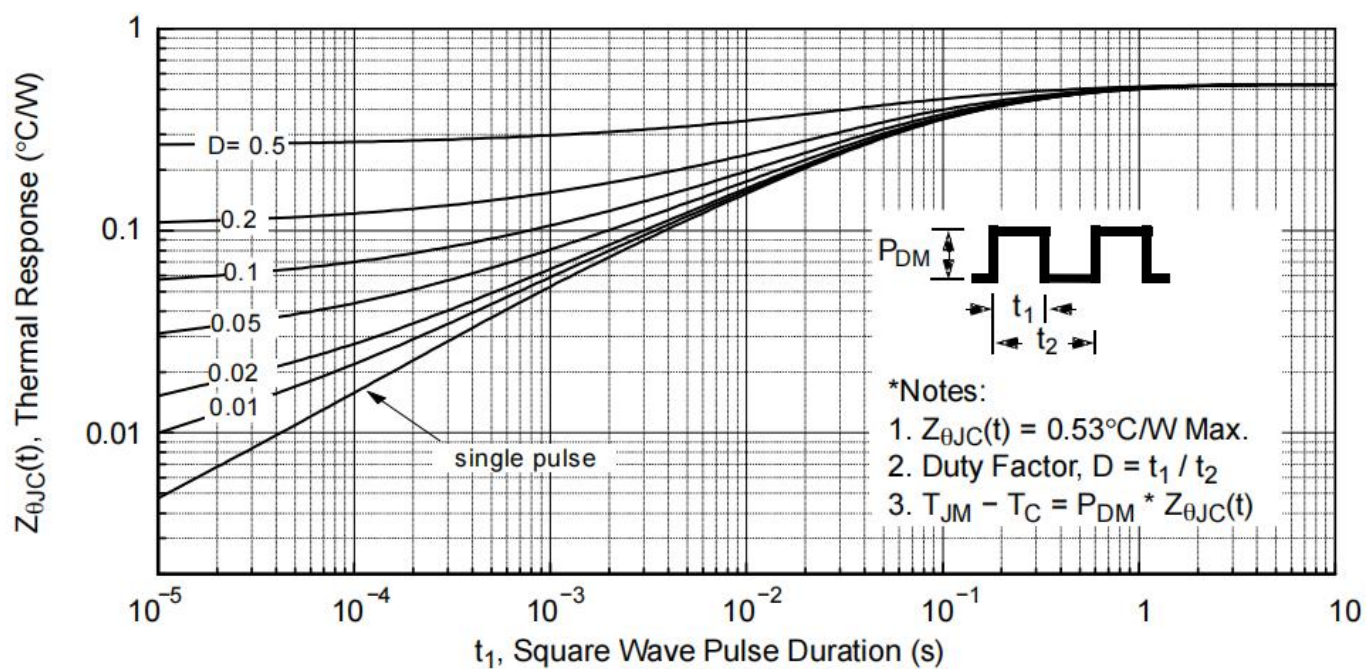
Fig 11: Max. Transient Thermal Impedance
