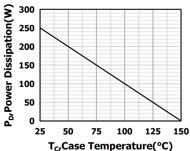
Fig 7: Power Dissipation
