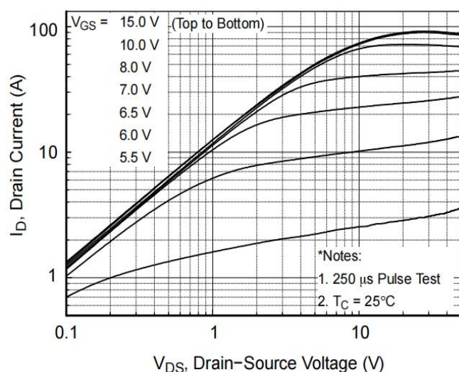
Fig 1: Output Characteristics
