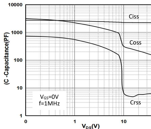
Fig 6: Capacitance Characteristics
