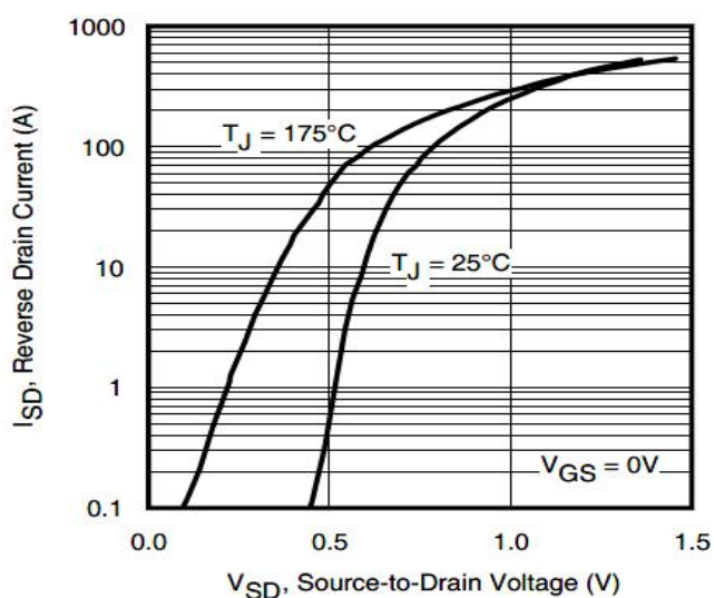
Fig 4: Body-diode Forward Characteristics
