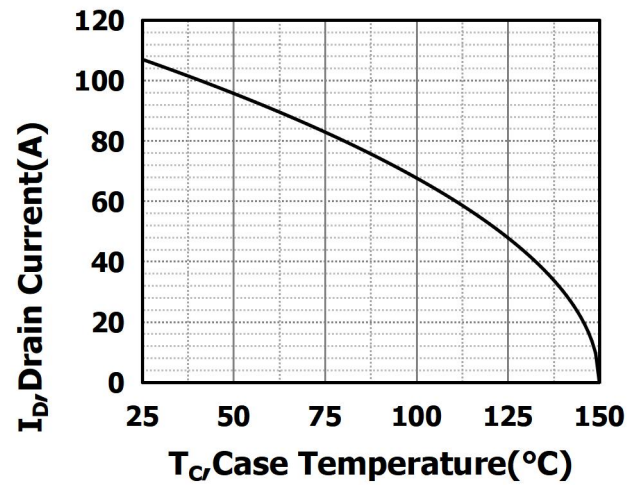
Fig 6: Drain Current Derating
