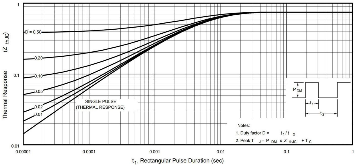
Fig10. Maximum Effective Transient Thermal Impedance, Junction-to-Case
