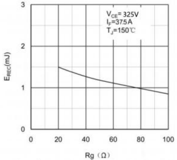
Figure 8. Switching Energy vs Gate Resistor Diode
