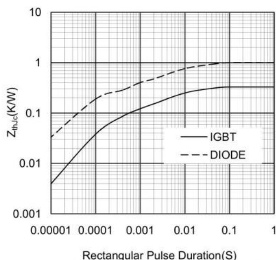
Figure 12. Transient Thermal Impedance of Diode and IGBT
