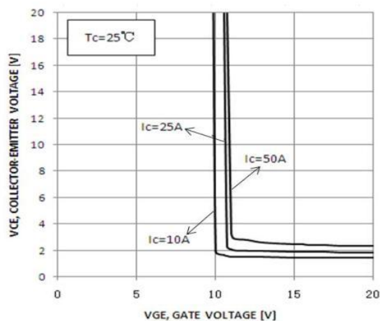
Figure 4. Typical Saturation Voltage vs. Gate-Emitter Voltage
