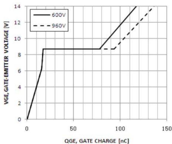
Figure 14. Typical Gate Charge
