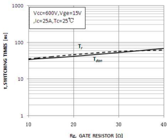
Figure 7. Typical Turn-On Characteristics vs. Gate Resistance
