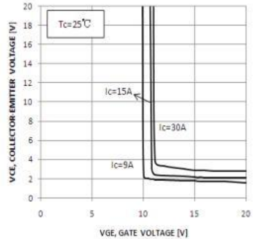
Figure 4. Typical Saturation Voltage vs. Gate- Emitter Voltage
