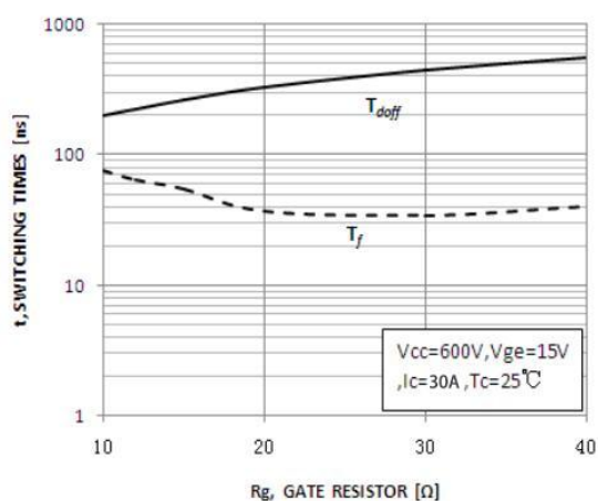
Figure 8. Typical Turn-Off Characteristics vs. Gate Resistance
