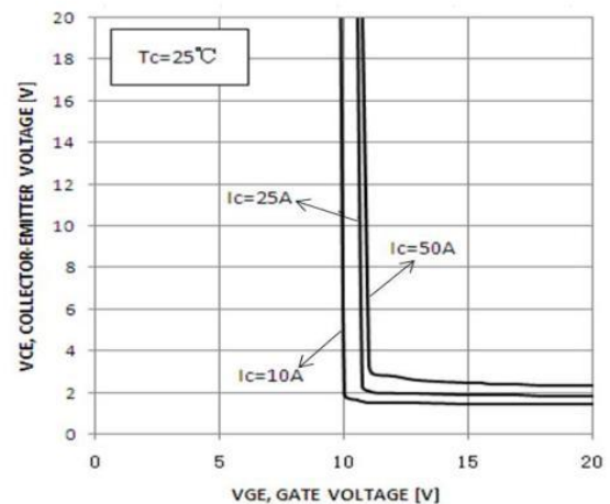
Figure 4. Typical Saturation Voltage vs. Gate-Emmitter Voltage
