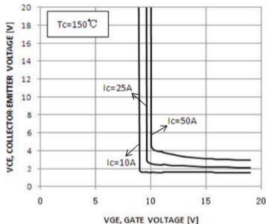
Figure 5. Typical Saturation Voltage vs. Gate-Emmitter Voltage
