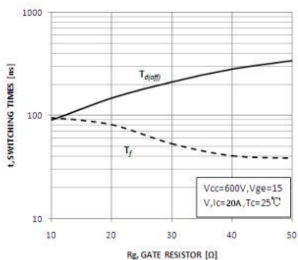
Figure 8. Typical Turn-Off Characteristics vs. Gate Resistance
