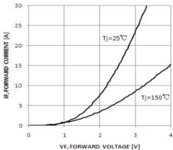
Figure 13. Typical Diode Forward Characteristics
