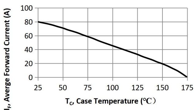
FIG.6 Average Forward Current vs. Case Temperature
