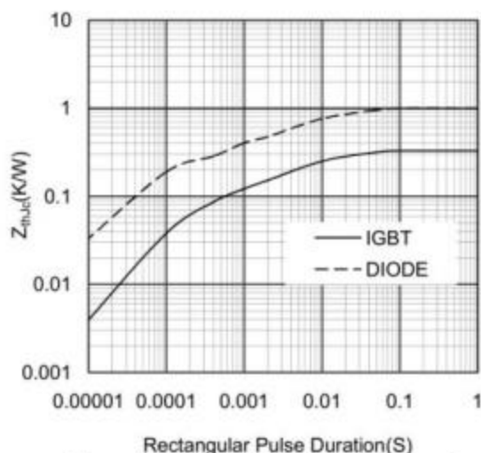
Figure 10. Transient Thermal Impedance of Diode and IGBT
