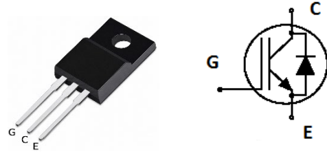
Package view and circuit symbol
