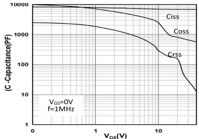
Fig 6. Capacitance Characteristics
