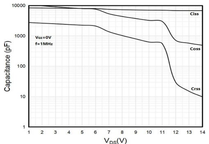
Fig 6. Capacitance Characteristics
