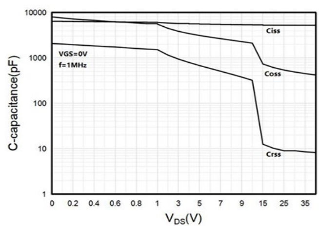
Fig 6. Capacitance Characteristics
