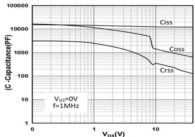
Fig 6. Capacitance Characteristics
