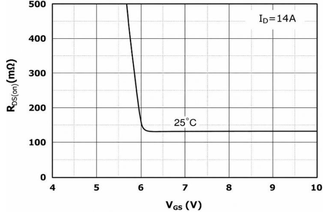
Fig 4. Rds(on) vs Gate Voltage
