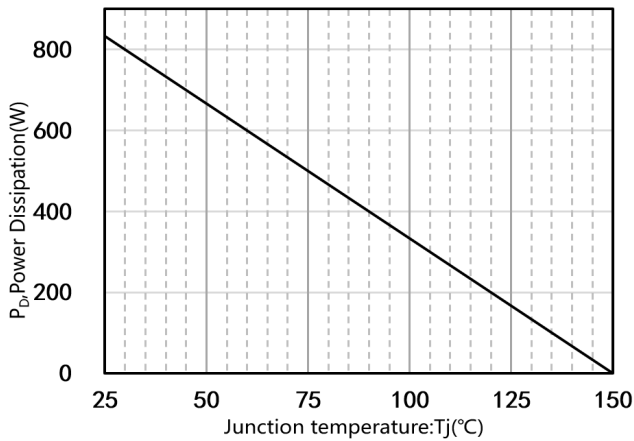
Fig 9. Power Dissipation
